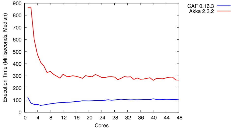
Bank Transaction (await infinite)
