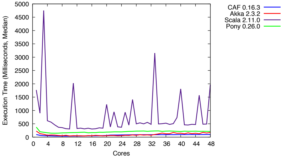
Bank Transaction (fastest implementations)
