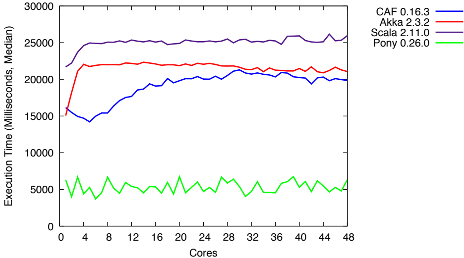
Concurrent Sorted Linked-List
