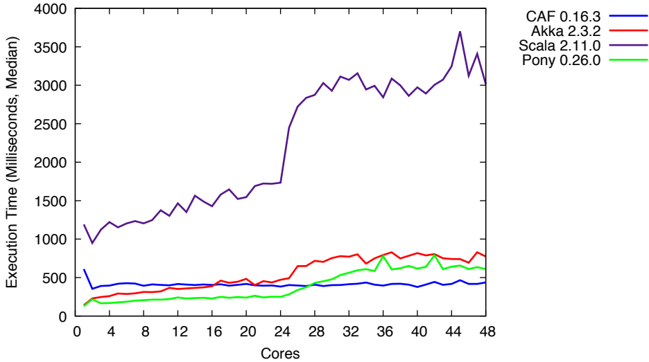
Dining Philosophers
