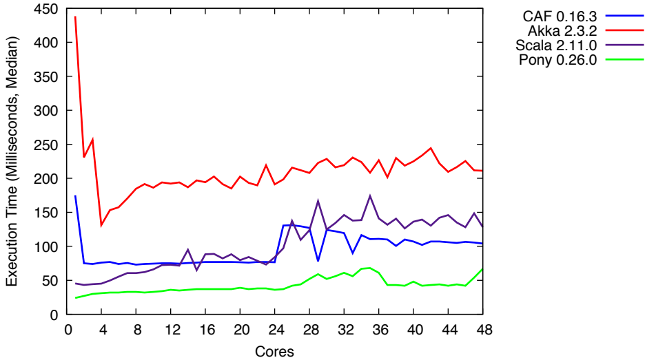
Fork Join (actor creation)
