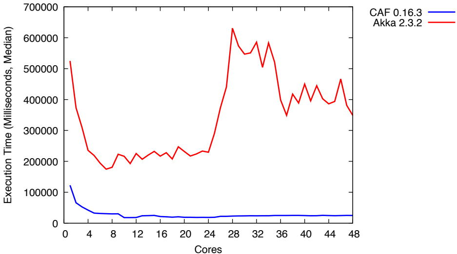
Logistic Map Series (unbecome slow)
