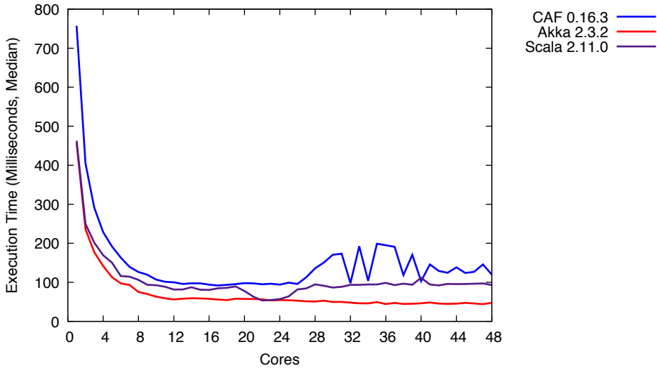
NQueens first K solutions
