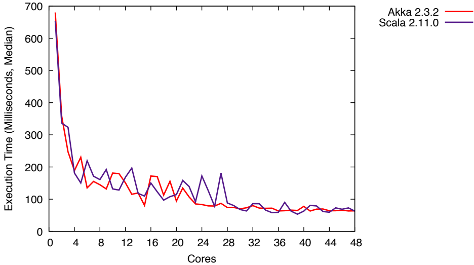
Precise Pi Computation
