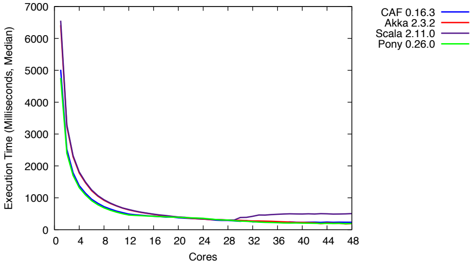
Producer-Consumer with Bounded Buffer
