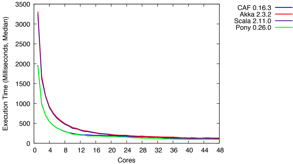
Trapezoidal Approximation
