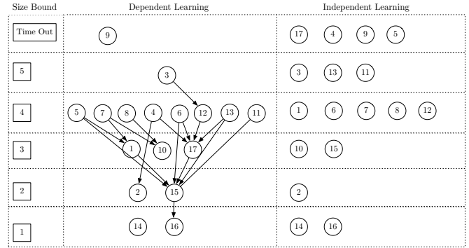
Figure 7. A comparison of the programs generated by Dependent and Independent Learning in a typical run of Metagol DF . Nodes marked n correspond to programs which solve task n , and nodes are arranged vertically according to their sizes. For Dependent Learning (left), the arrows correspond to the calling relationships of the induced programs.
