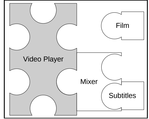
Figure 3: Non-determinism
